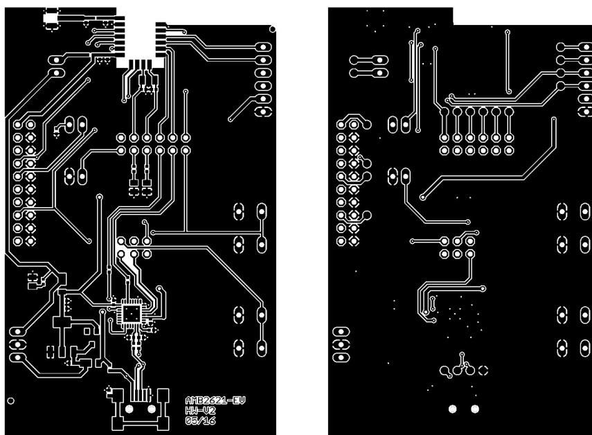
Figure 17: Top & bottom Layer
