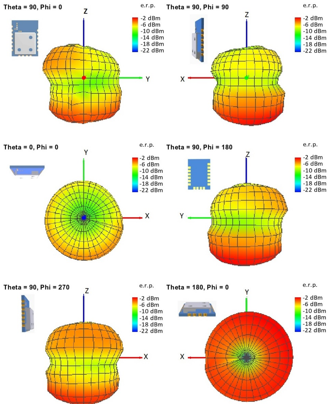
Figure 18: Antenna characteristic from integrated antenna measured on official EV-Board*
