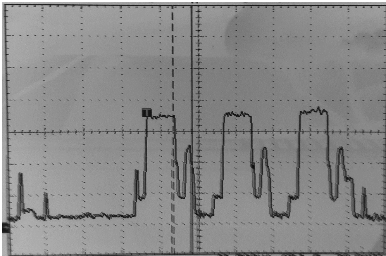
Figure 4: Measured Proteus-II transient current consumption in advertising mode with 40 ms advertising interval, excerpt of 5ms
