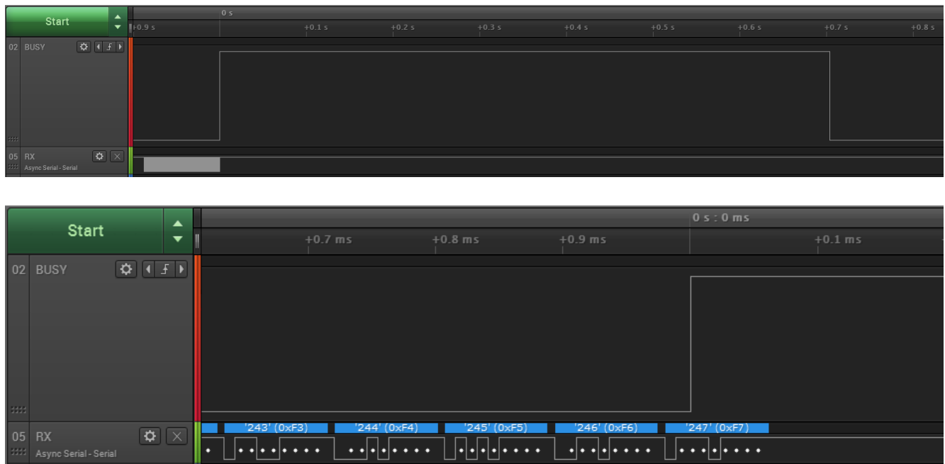
Figure 9: Switch of the BUSY pin when transmitting data
